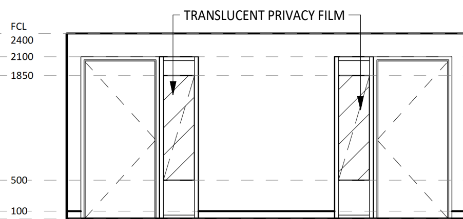
5 ELEVATION DETAIL 1 : 50
