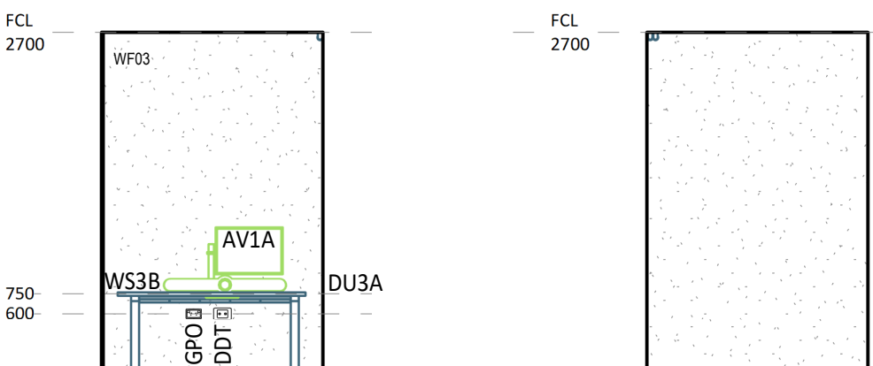
7 ELEVATION DETAIL 1 : 50
